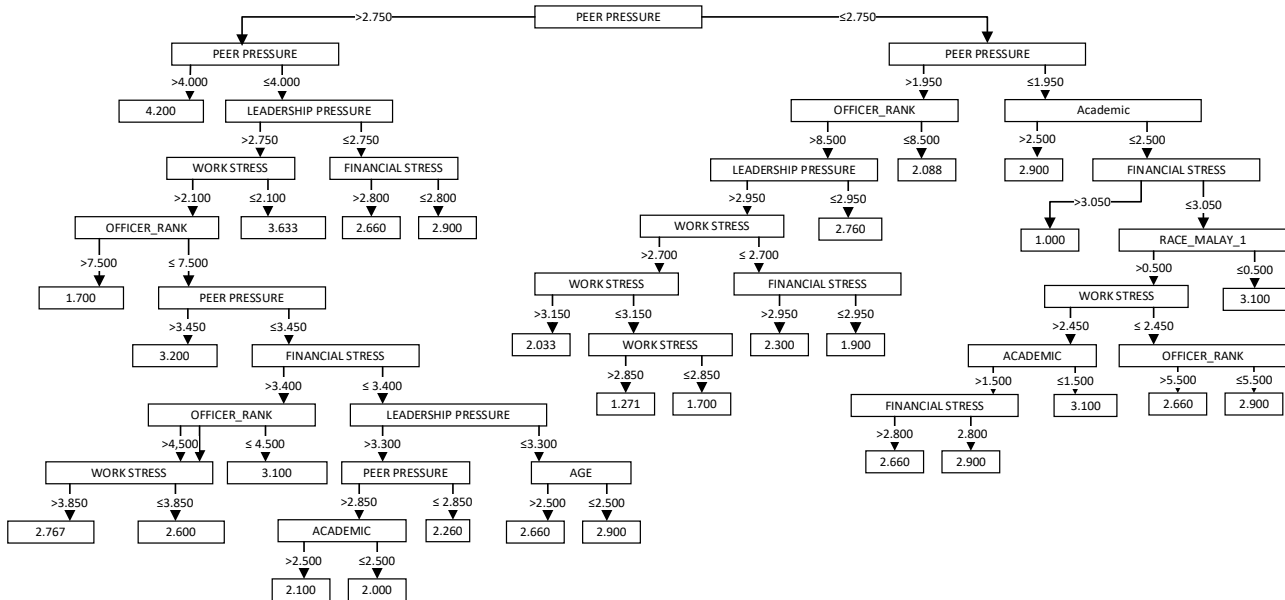
Fig. 6: The tree model from the decision tree
